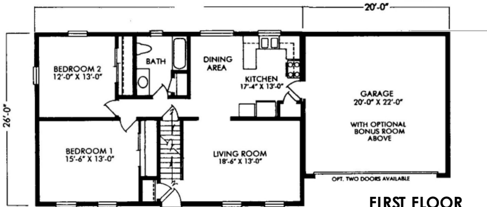
FIRST FLOOR 1040 SF
